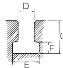
T溝寸法図 T-slot dimensional drawing
