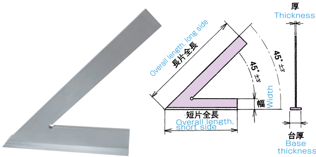
●OS-156A 寸法表 Dimensions OS-156A
