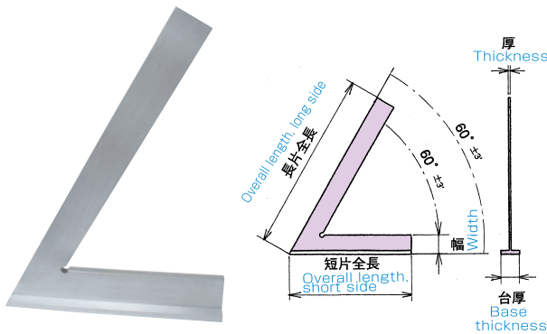
●OS-156C 寸法表 Dimensions OS-156C
