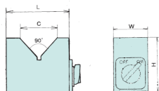
●OS-128MG 寸法表 Dimensions OS-128MG
